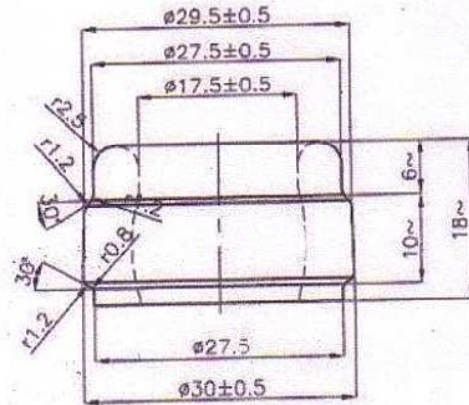
Detail of finish M2:1
